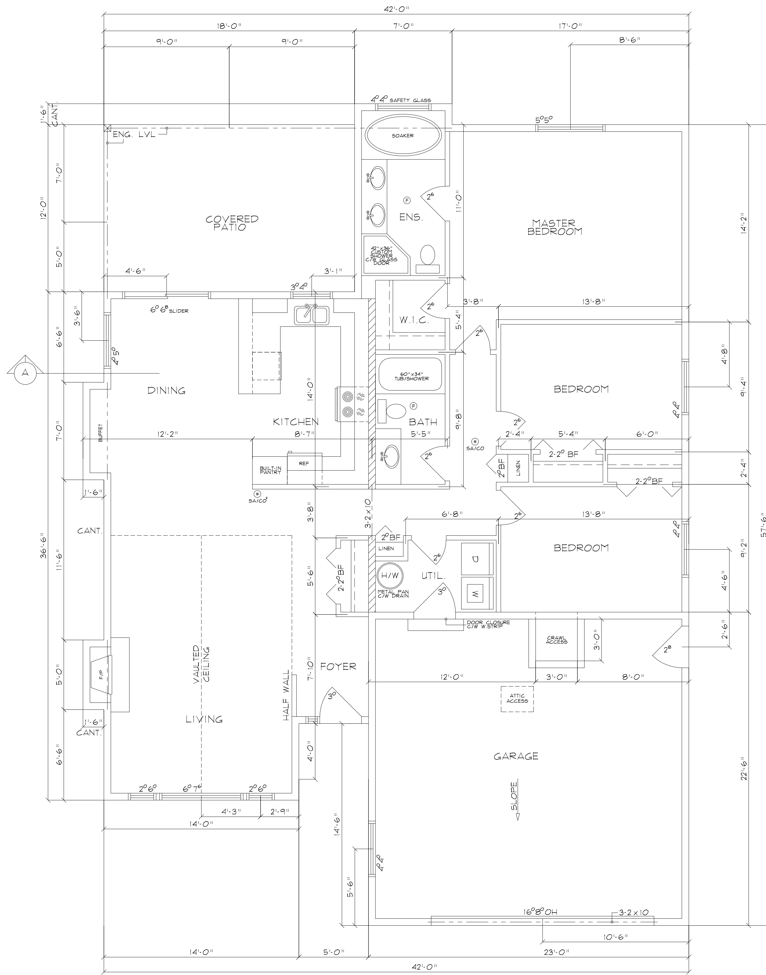
FLOOR PLAN 1/4" = 1'-0" 1519 SQ/FT
